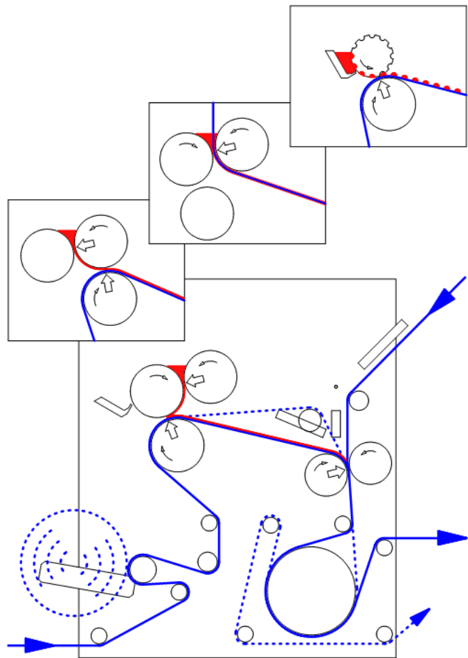
Multi Roll Both side Coating
