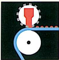
CAVISCREEN rotary screen coating
